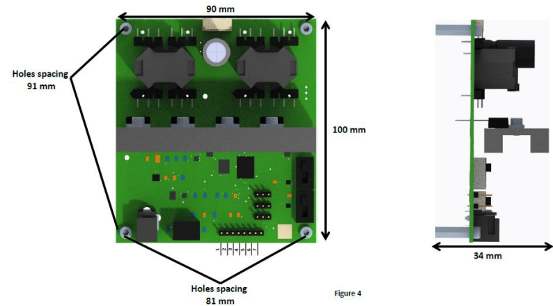
Board dimensions
