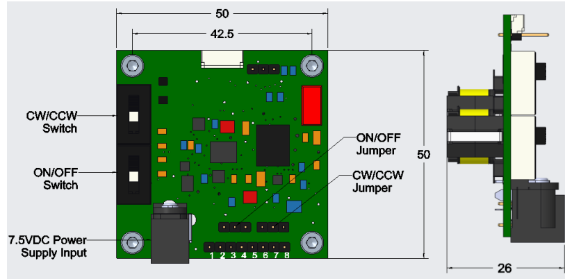
BOARD DIMENSIONS
