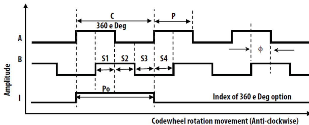
QUADRATURE SIGNALS A, B and I
