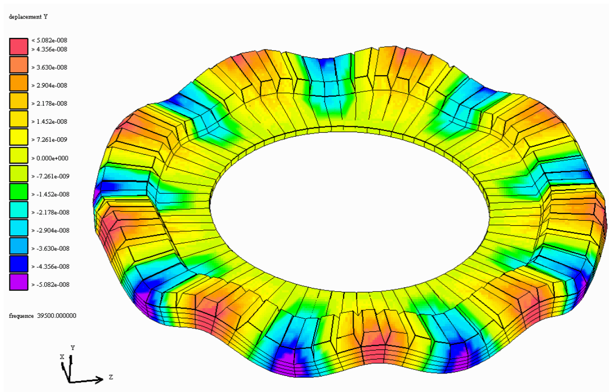
SIMULATION OF TRAVELLING WAVE MODULATION ON A WLG-75 STATOR
